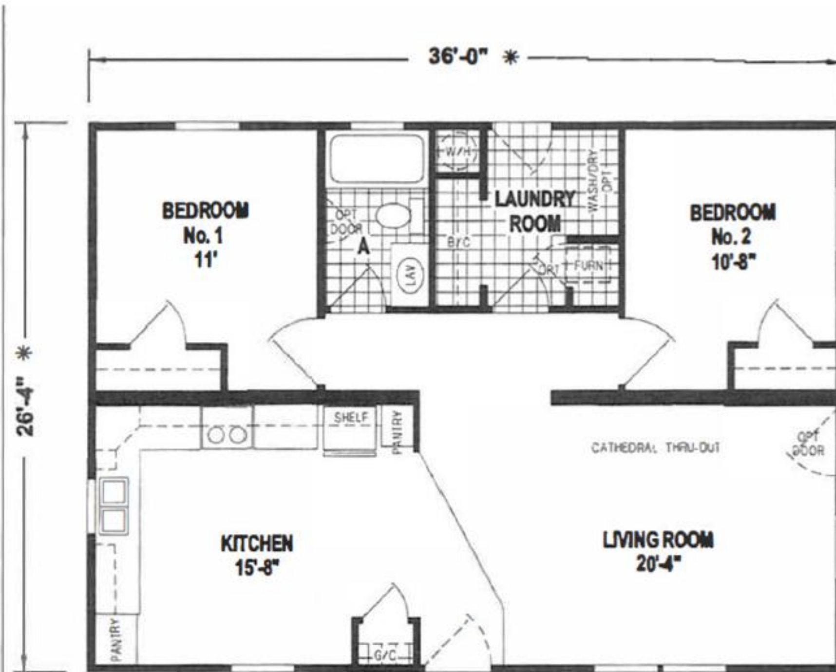
A234CTG/3628 (948 SQ. FT.) 2BEDROOM - CATHEDRAL THRU-OUT
